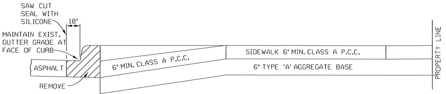
DRIVEWAY SECTION
