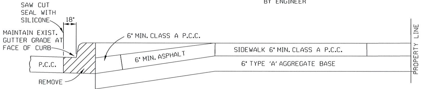
DRIVEWAY SECTION
