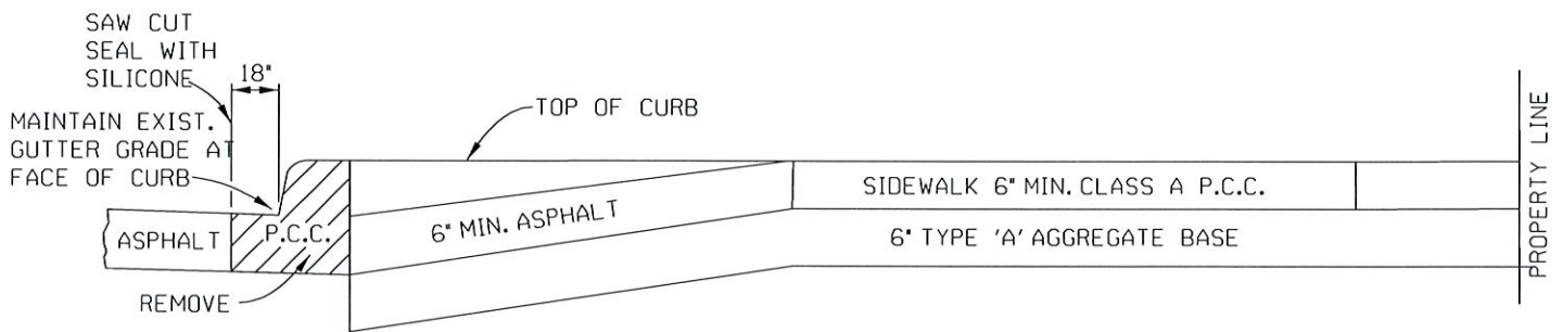
DRIVEWAY SECTION
