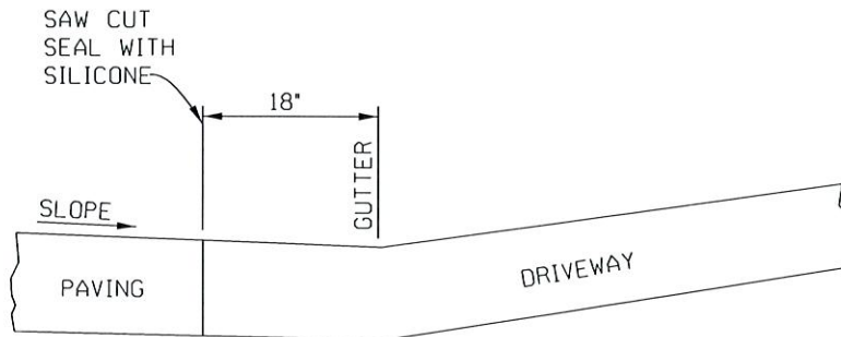
DRIVEWAY SECTION
