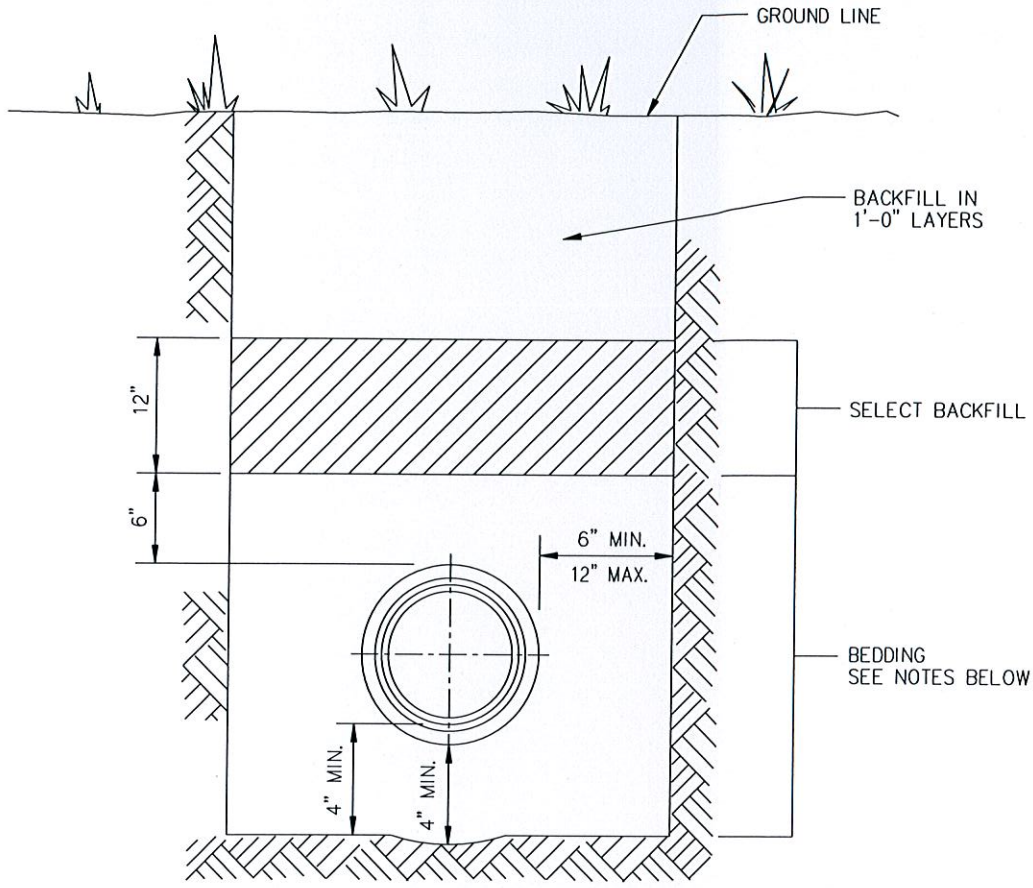
TRENCH CROSS-SECTION
