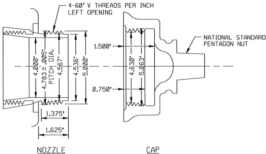
TULSA STANDARD THREADS - PUMPER NOZZLE
