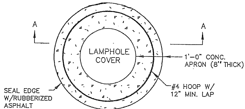
PLAN VIEW
