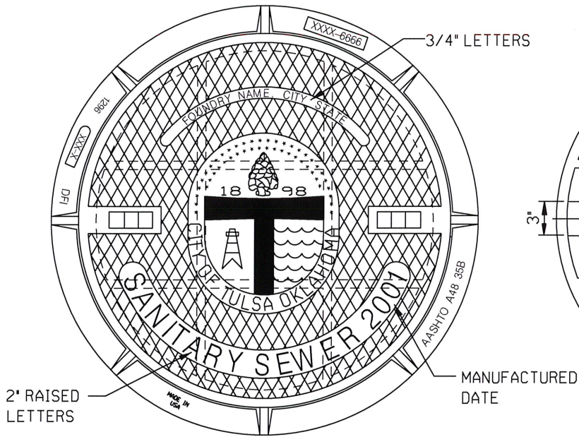
LID AND FRAME - TOP VIEW
