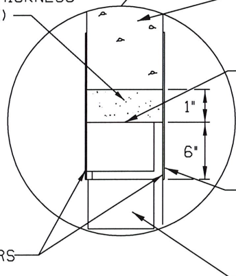
CORBEL (CONE) REPLACEMENT DETAIL NOT TO SCALE
