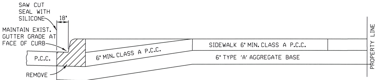
DRIVEWAY SECTION
