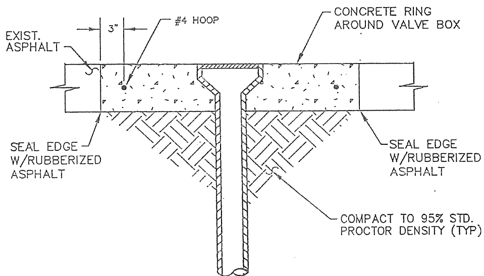
SECTION A
