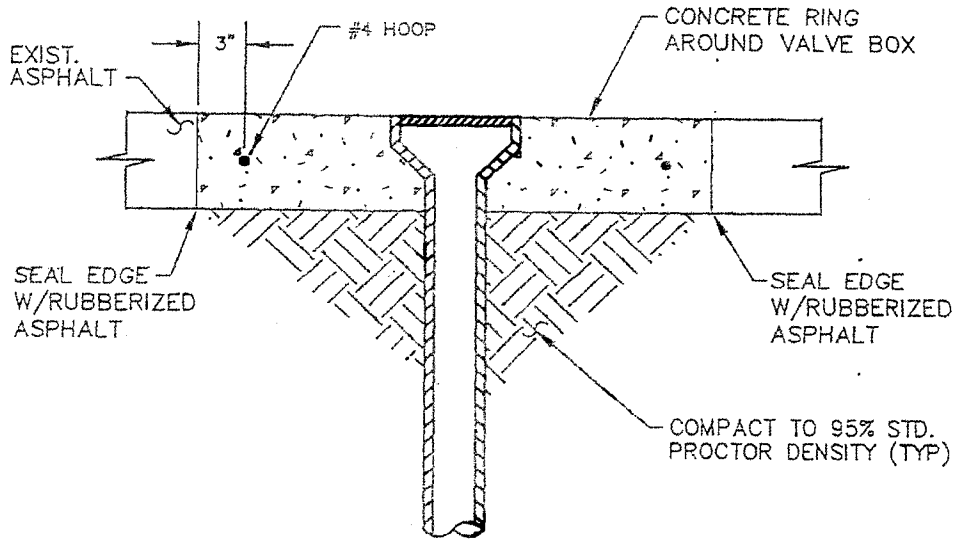
SECTION A
