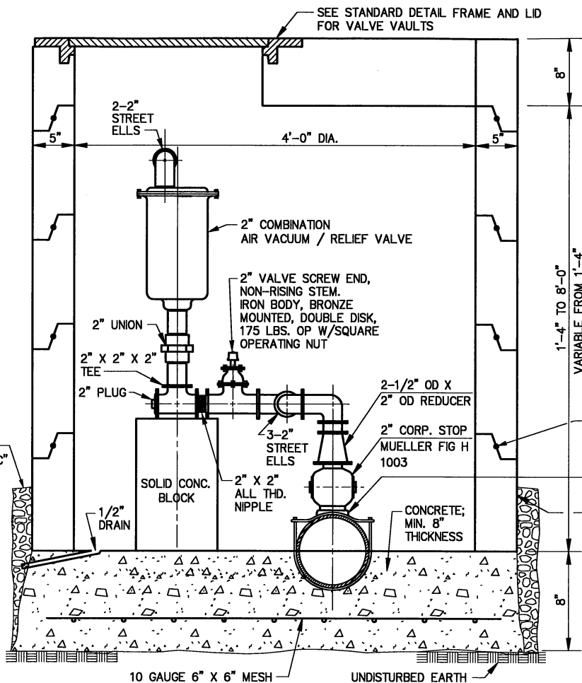
REINFORCED CONCRETE VAULT ALTERNATE FOR STREET TRAFFIC
