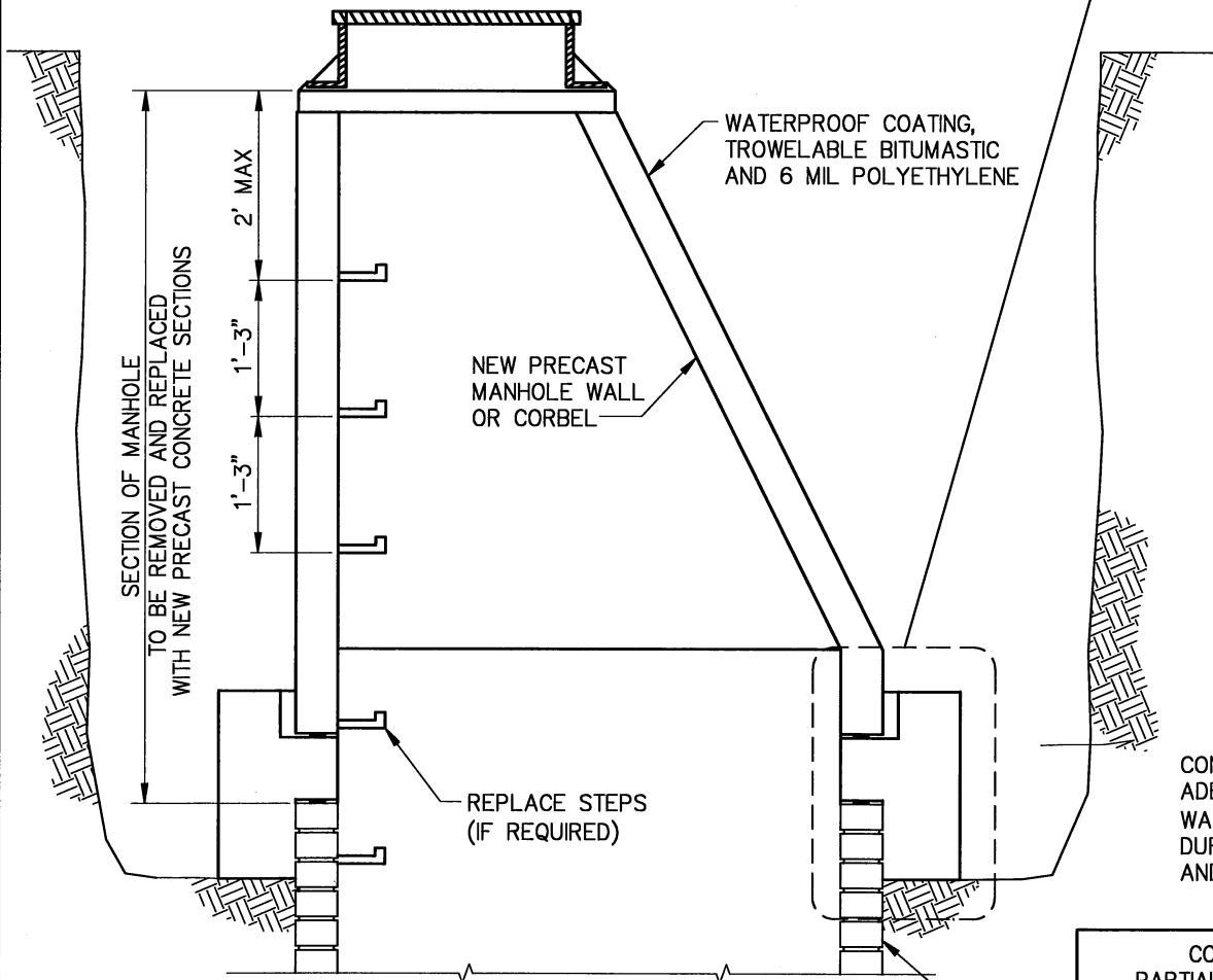
PARTIAL MANHOLE REPLACEMENT TYPE F REPAIR NOT TO SCALE
