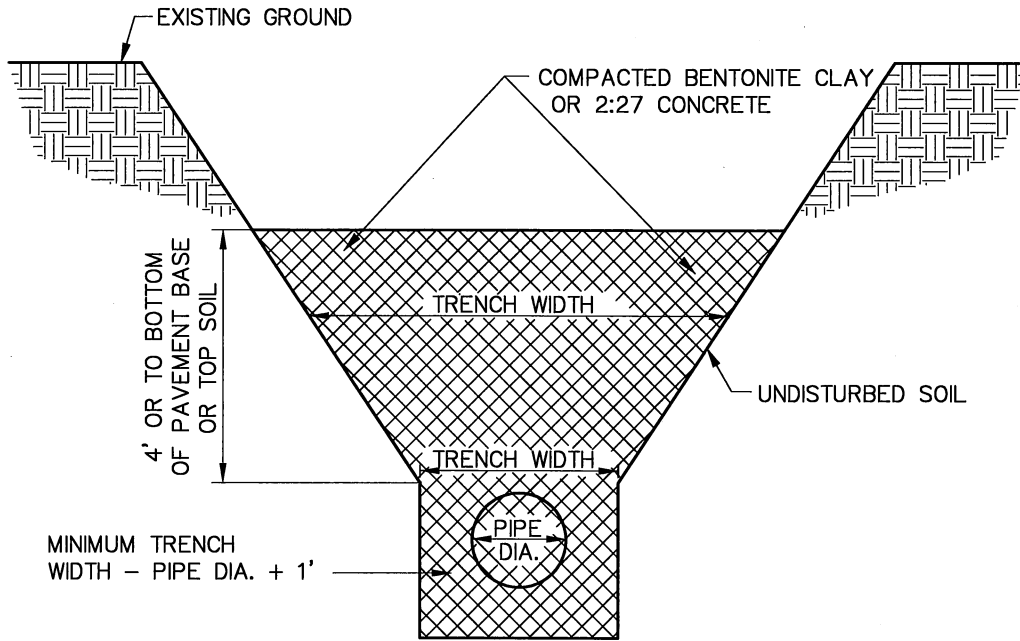
CLAY DAM SECTION
