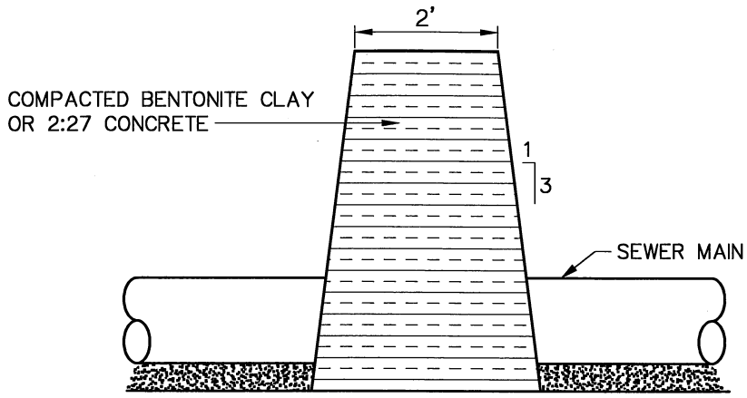
CLAY DAM PROFILE
