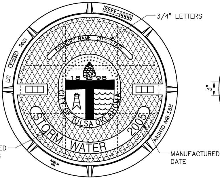
LID AND FRAME - TOP VIEW
