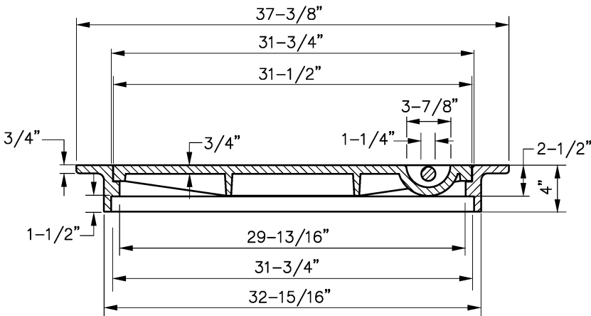
LID AND FRAME
