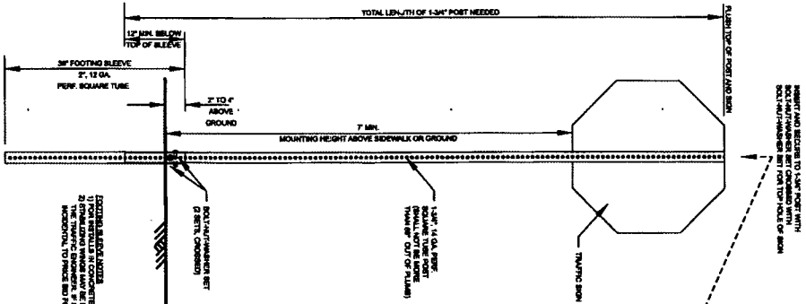
SIGN INSTALLATION DETAIL
