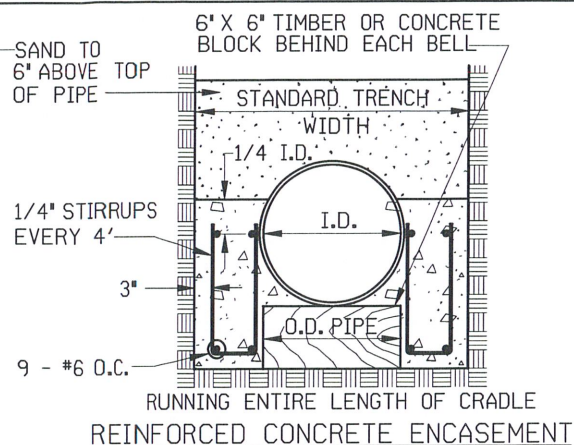
REINFORCED CONCRETE ENCASEMENT
