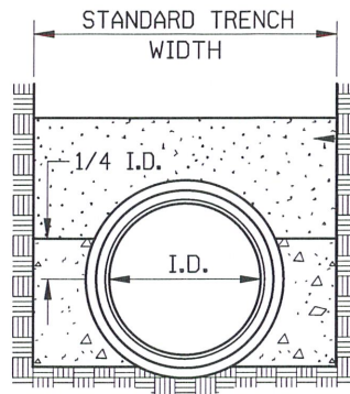
CONCRETE CRADLE
