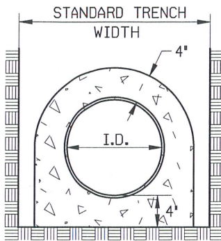
CONCRETE ENCASEMENT
