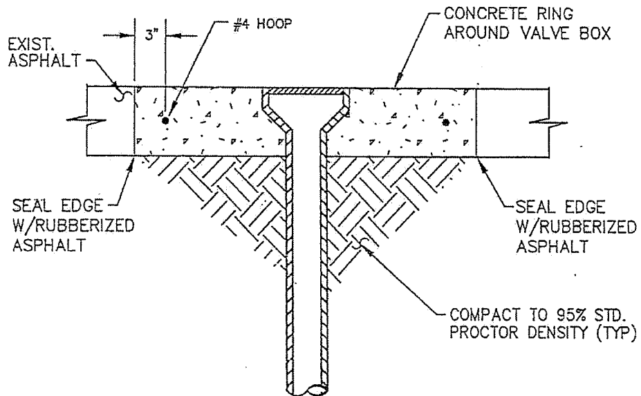
SECTION A
