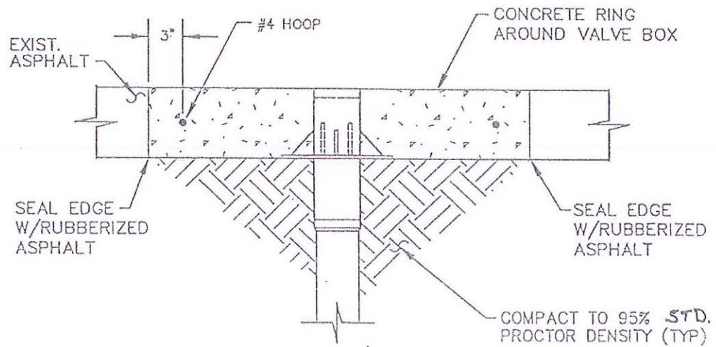
SECTION A
