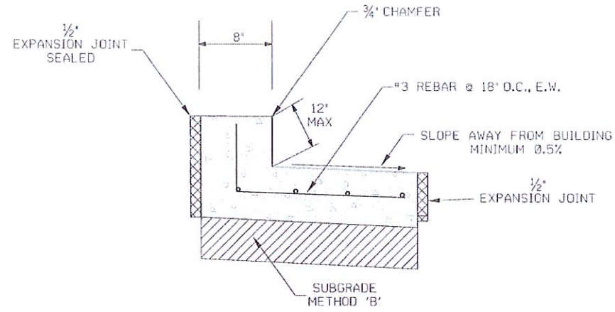
INTEGRAL SIDEWALK CURB
