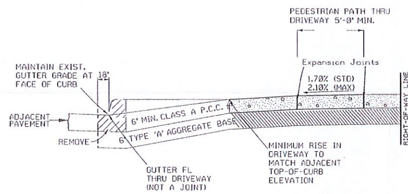
DRIVEWAY SECTION Section A-A (At Centerline)
