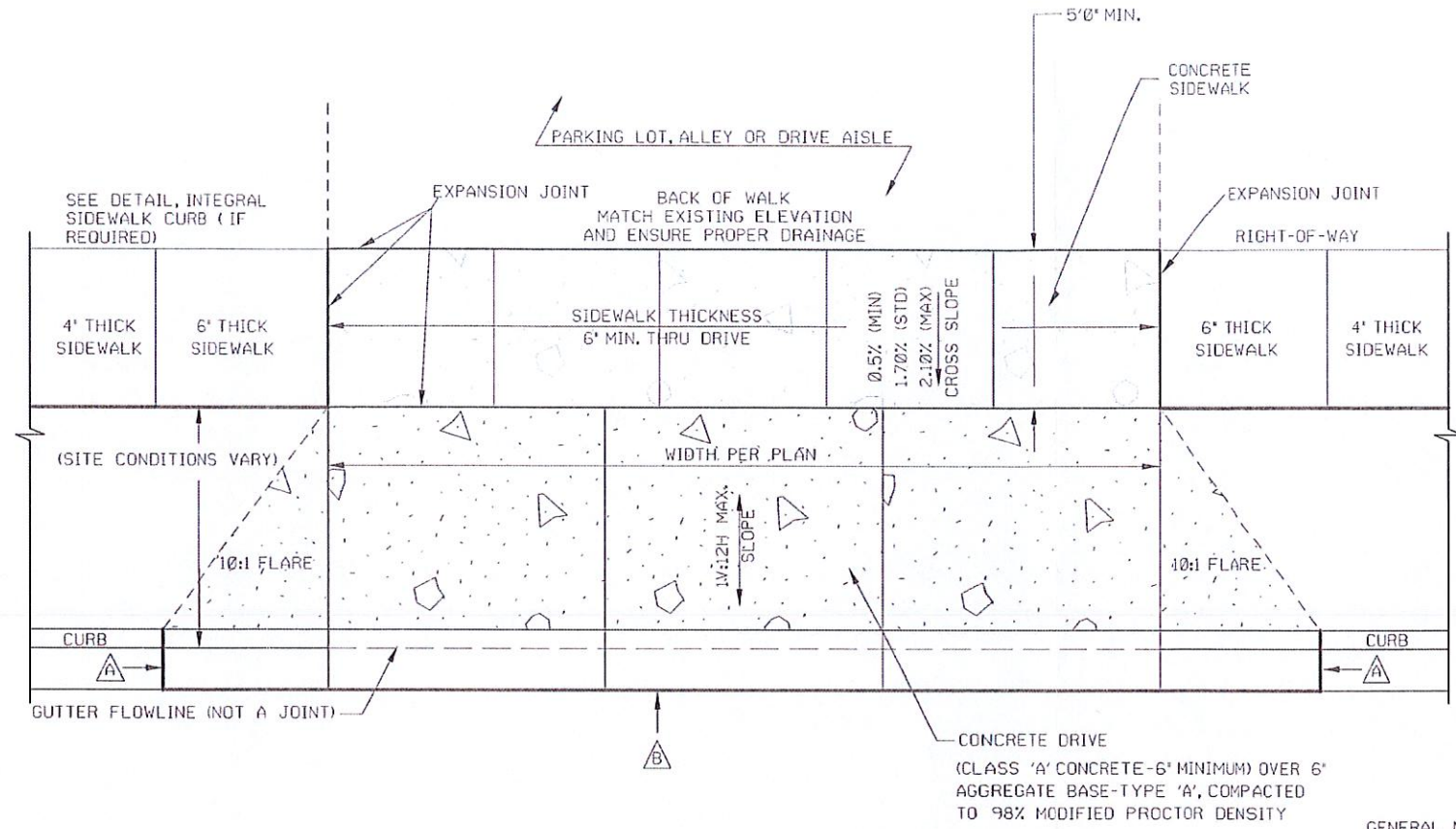
DRIVEWAY DETAIL 3
