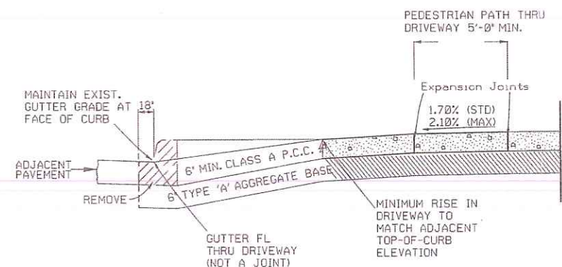
DRIVEWAY SECTION Section A-A (At Centerline)
