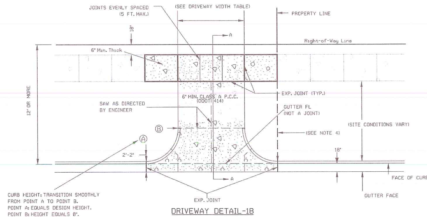
DRIVEWAY DETAIL-1A (For Use on Curbed Concrete Streets)
