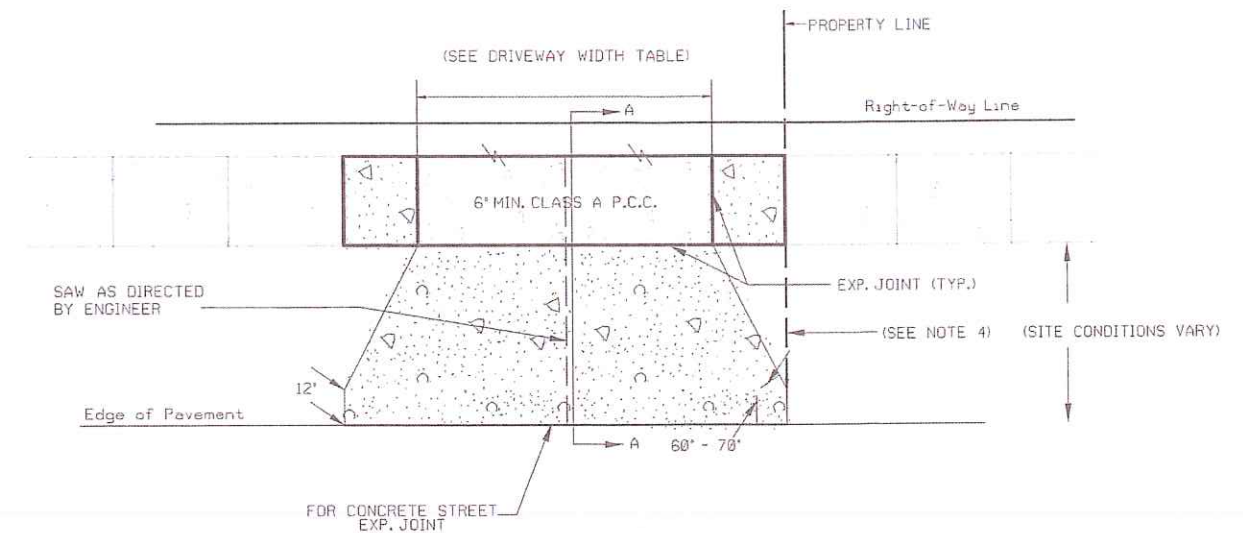
DRIVEWAY DETAIL-2 (For Use on Un-Curbed / Ditched Streets)
