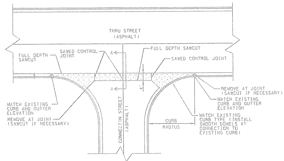
CROSS STREET CONCRETE GUTTER DETAIL
