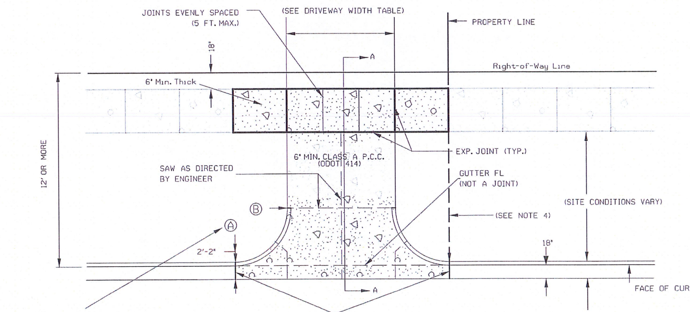
DRIVEWAY DETAIL-1B (For Use on Curbed Asphalt Streets)
