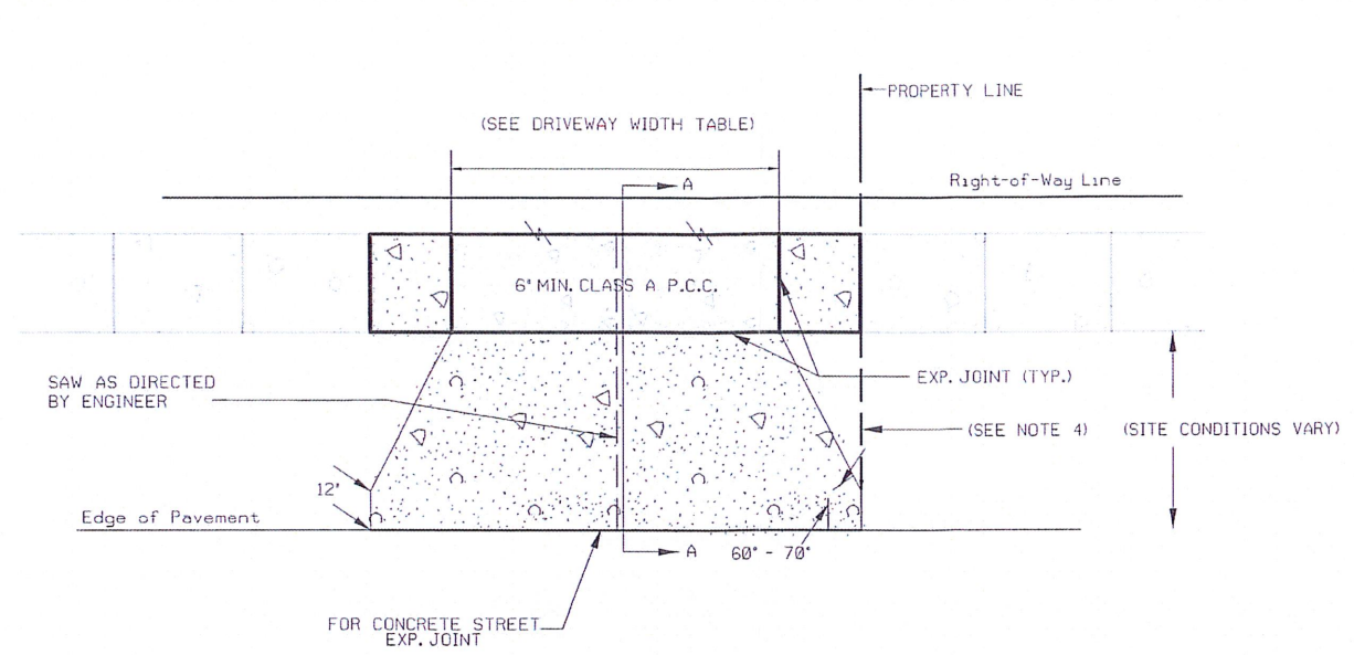
DRIVEWAY DETAIL-2 (For Use on Un-Curbed / Ditched Streets)
