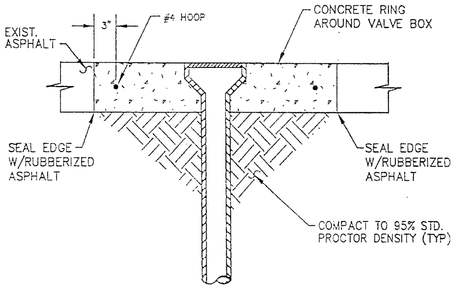
SECTION A
