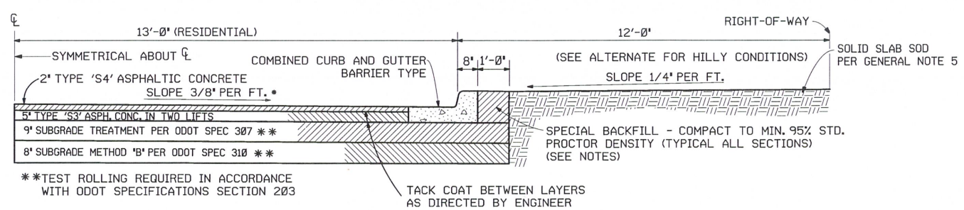
TYPICAL HALF SECTION - SECTION 1 SN > 3.50 INTERIOR, NON-COLLECTOR
