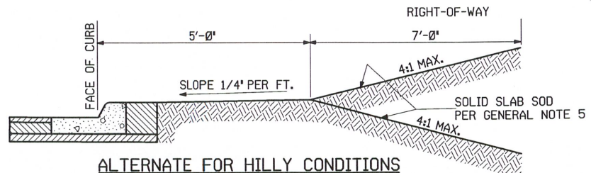
ALTERNATE FOR HILLY CONDITIONS
