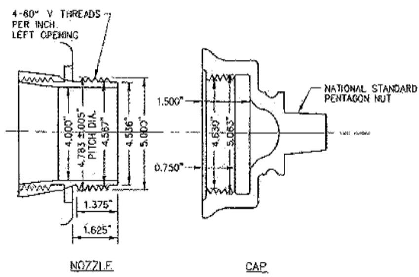
TULSA STANDARD THREADS-PUMPER NOZZLE
